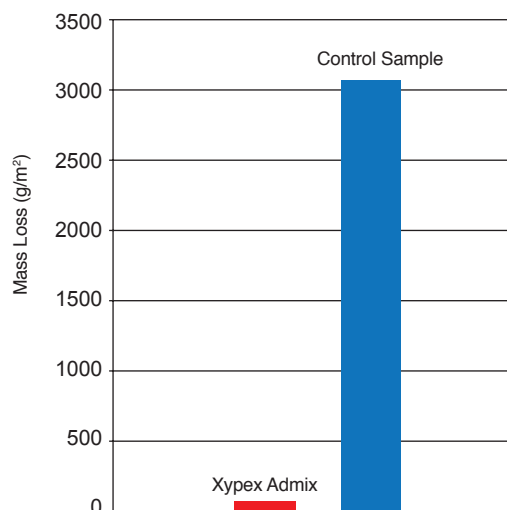
Accelerated sulfate corrosion test results.
