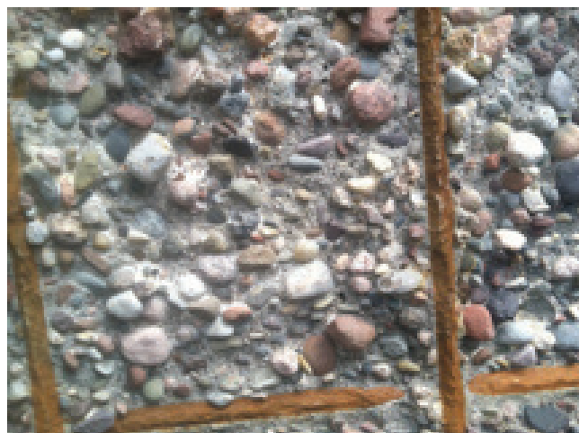
MIC deterioration at a wastewater treatment plant intake structure with a loss of approximately 2" of concrete.
