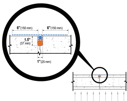
Details for crack or joint sealing (against a flow of water)
